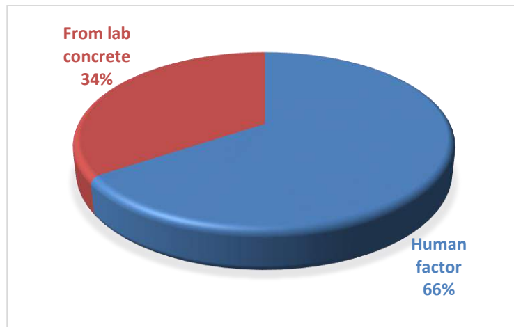
Figure 2.5: Outside Scope
