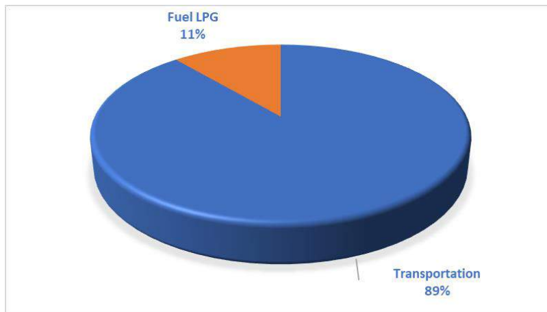
Figure 2.3: Scope 1 Emissions
