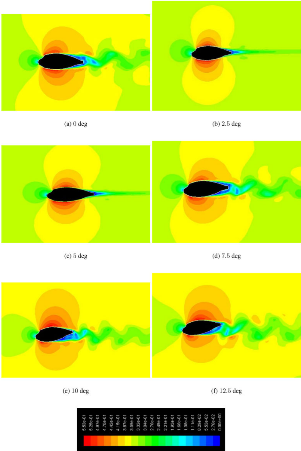
Figure 9. Velocity contours around the UUV at various angles of attack.
