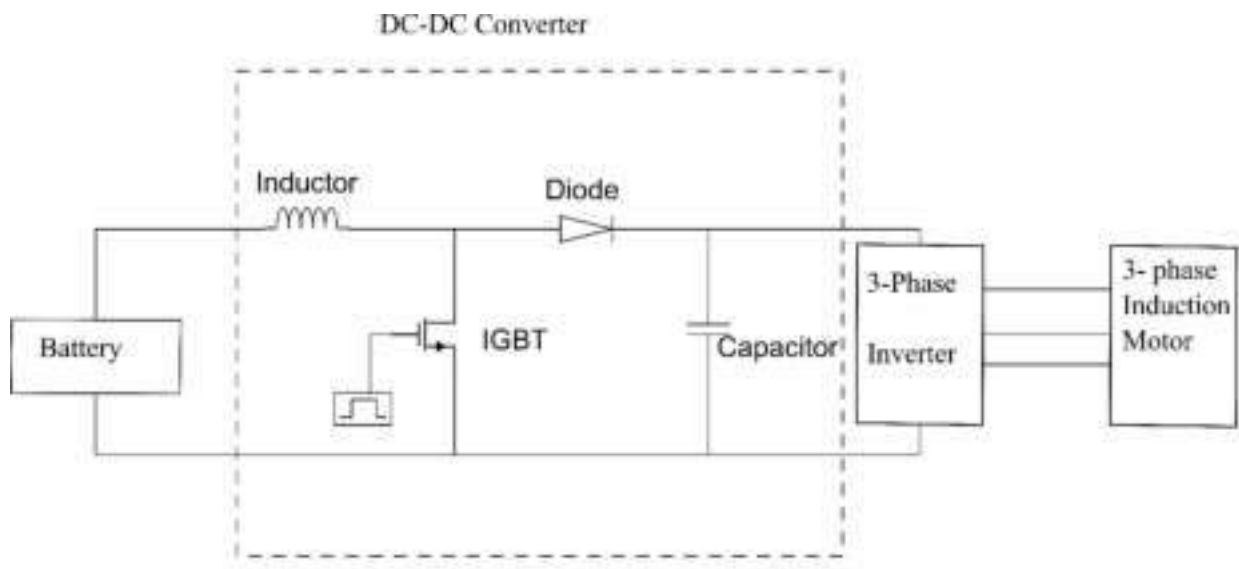
Fig 2.2 Schematic circuit diagram of electric propulsion for boat
